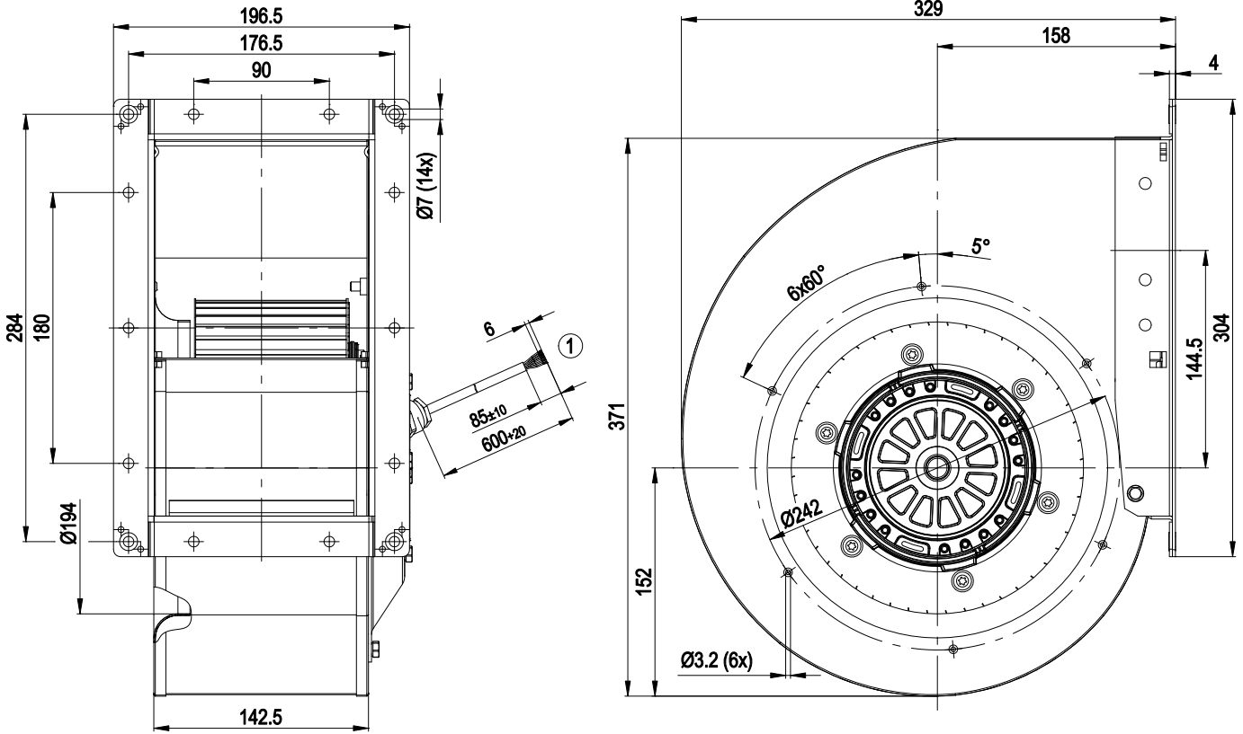
1 Connection line silicone, 6x brass lead tips crimped
