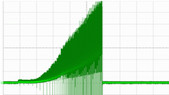
Locked rotor current @ 72 V (I = 200mA/div ; t = 500ms/div)
