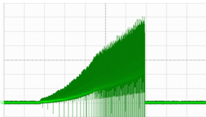
Locked rotor current @ 36 V (I = 200mA/div ; t = 500ms/div)
