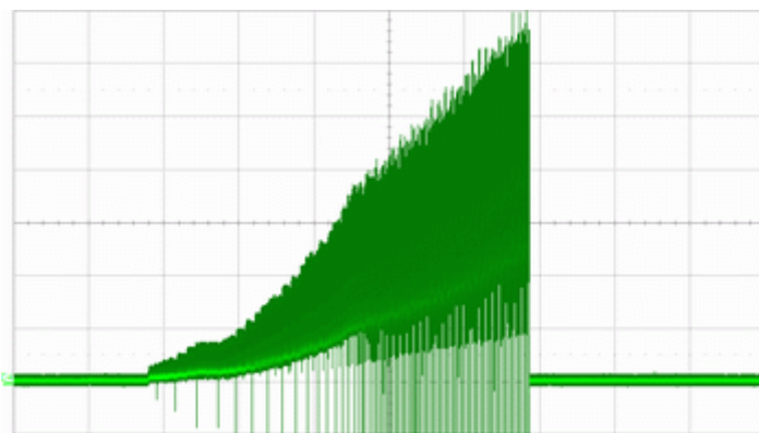
Locked rotor current @ 48 V (I = 200mA/div ; t = 500ms/div)
