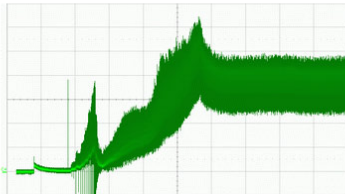
Start-up current @ 48 V (I = 200mA/div ; t = 2s/div)
