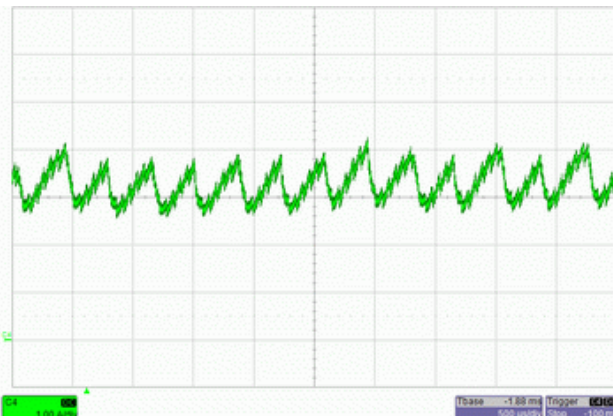
Running current @ 48 V ( I = 1 \text{ A/div} ; t = 500 \mu\text{s/div} )
